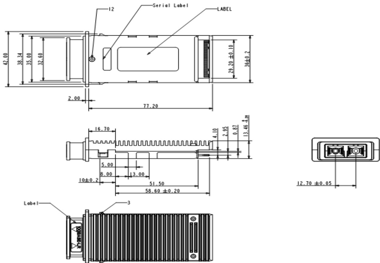
Figure3. Mechanical Dimensions
