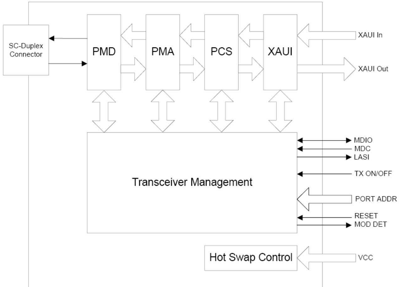
Figure2. Functional Diagram of Typical X2 Style Transceiver
